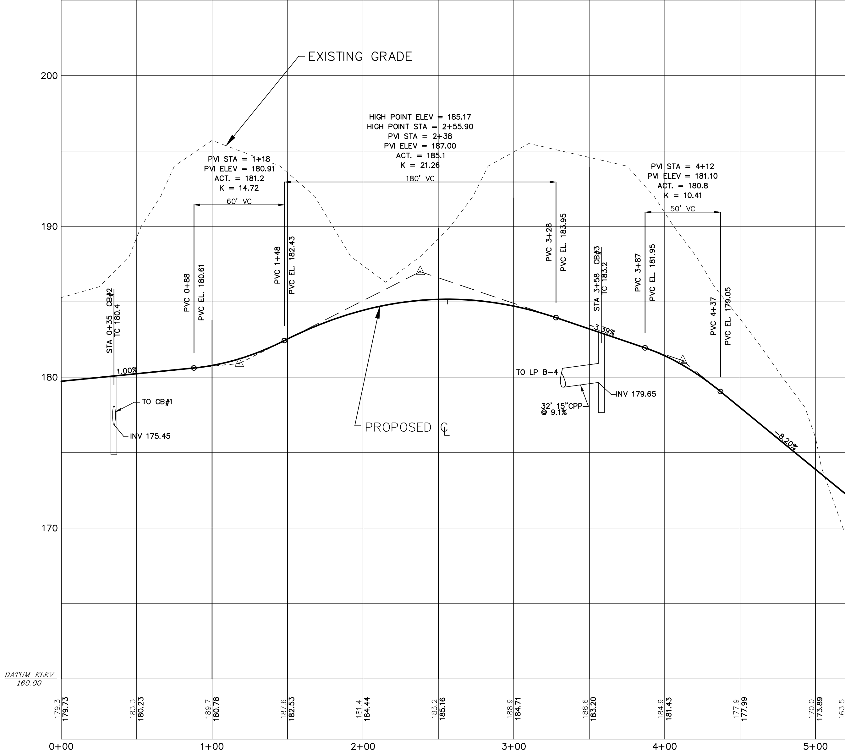
THERESA SOUTH SCALE: HORIZ. 1"=40' VERT. 1"=4'
